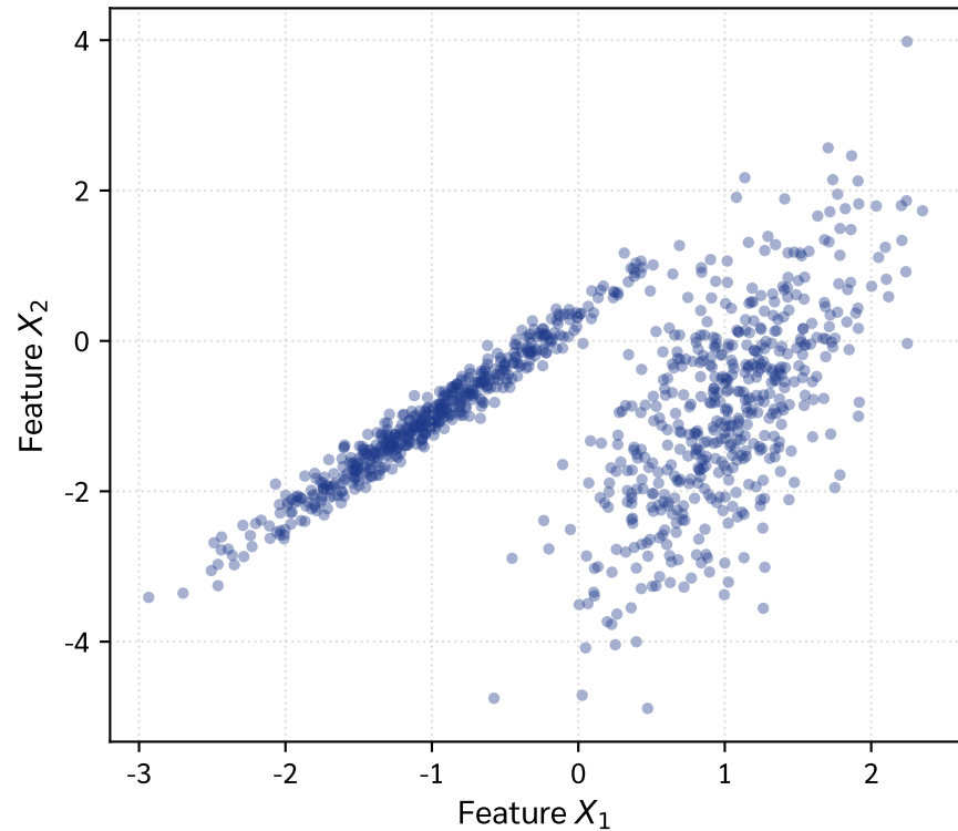
(a) Dataset 4: Anisotropic Blobs ( N = 1000 )
