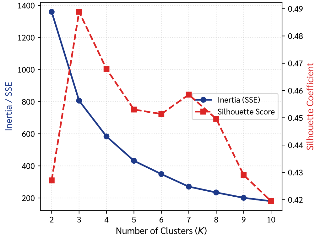
(b) Metric Curves ( K = 2 \dots 10 )
