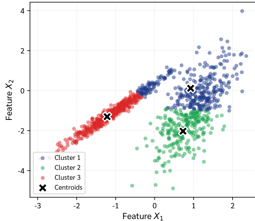
(c) K-Means Result ( K = 3 , Peak Sil=0.489)
